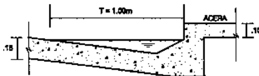
CUNETA TRIANGULAR
